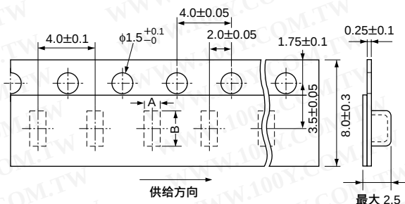
8mm 宽, 4mm 间距编带
